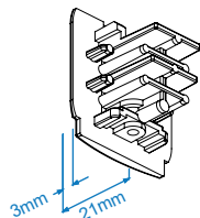
Tapa final ciega carril JA113
