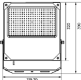
F901CCT 120-150-200W
