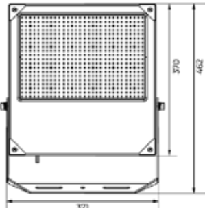
F902CCT 200-240-300W
