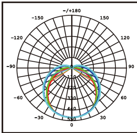
20W Photometric
