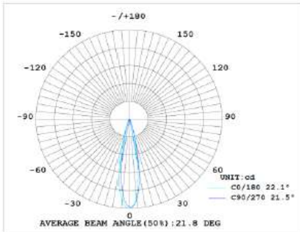
20° PC lens
