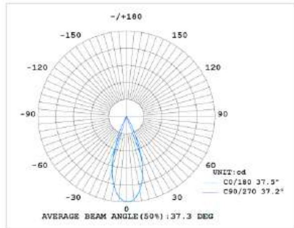
40° PC lens
